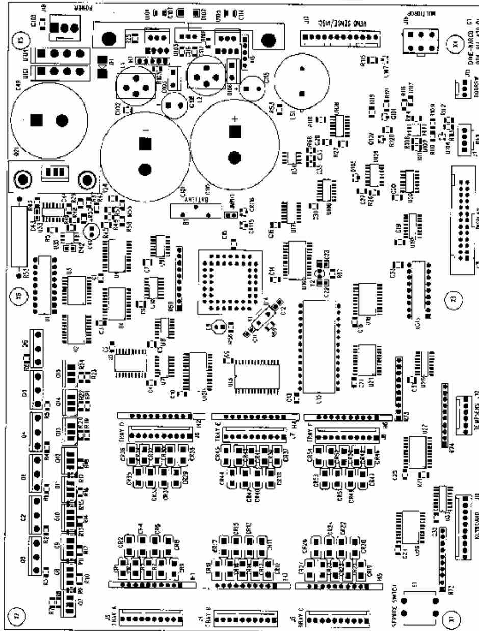
FIGURE 2 – MDB CONTROLLER CONNECTIONS DN 59## / 54## / 39## SERIES
