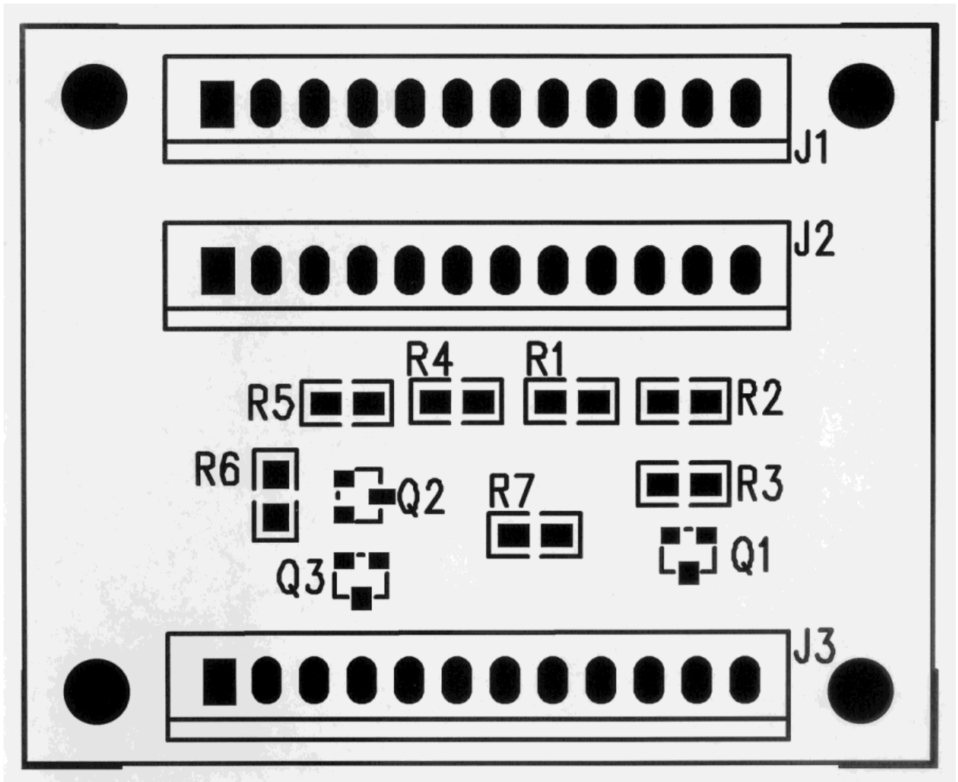
DUAL SENSOR BOARD (NON ENERGY STAR)
